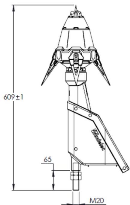
Dimensions (mm)
